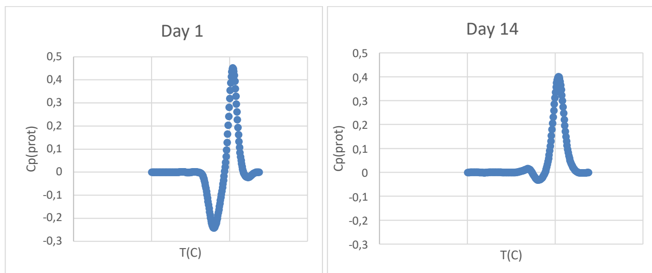
Fig 3. The DSC melting curves of glycated by lactose Cyt C in 0.15 M NaCl + 20 mM PBS + 2 mg/mL Cyt C + 0.55 M lactose solution at different stages of the glycation process. Left-Day 1; Right- day 14.
