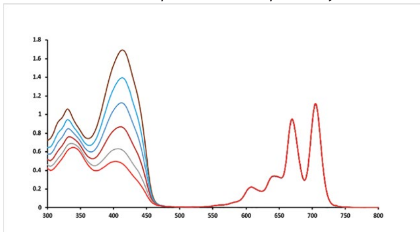
SCHEME 2. Singlet oxygen production of compounds
