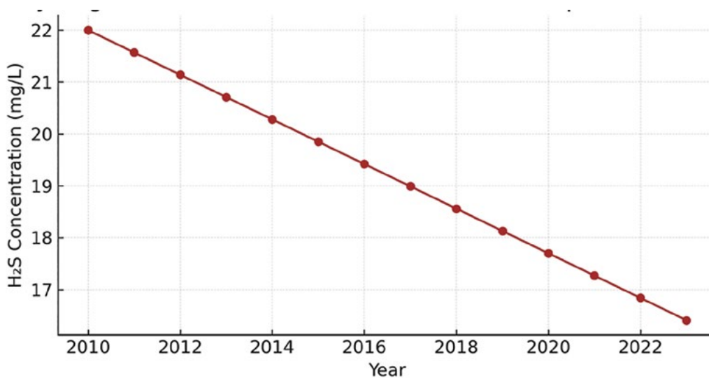
Figure 5. Hydrogen Sulfide ( H_2S ) Concentration in Therapeutic Muds (2010–2023).
